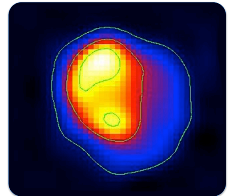
5 GHz raw map of the supernova remnant 3C157/IC443, obtained with the Medicina 32-m dish. Courtesy of Alberto Pellizzoni et al. (2013).
